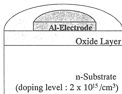
Fig. 1. Schematics illustration of the MOS capacitor sample
