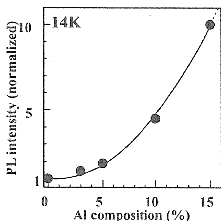
Fig.4 PL intensity related to \text{Tb}^{3+} emission as a function of Al contents in AlGaIn.
