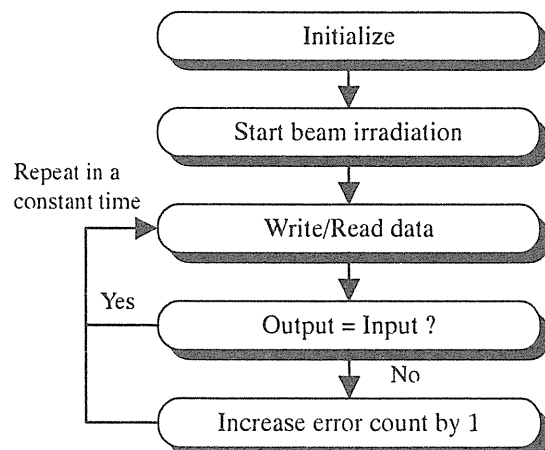
Figure 2. Measurement procedures.
